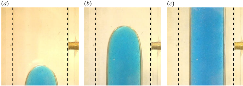
Figure 19. Experiment 2 (see table 1 ) with inner ascending and outer descending Newtonian fluids. Here, \mathcal{R} = 0.796 , Ar = 1.11 , \mathcal{M} = 10^3 , Bm = 0 . Three snapshots at different stages of the current evolution are shown.
