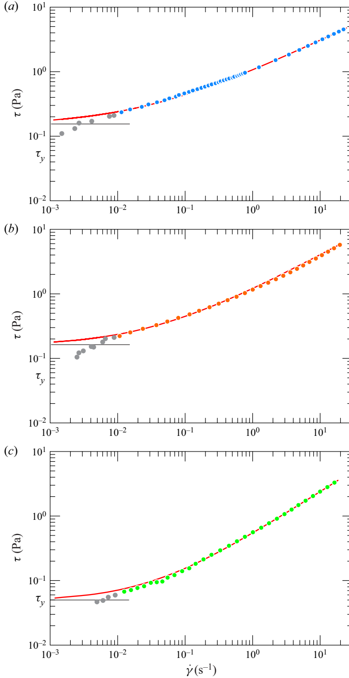
Figure 27. Flow curves for the HB fluids, (a) for experiment 9, with \tau_y = 0.15 Pa, n = 0.50 , \mu_0 = 0.92 Pa s n ; (b) for experiment 10, with \tau_y = 0.16 Pa, n = 0.56 , \mu_0 = 1.06 Pa s n ; (c) for experiment 11, with \tau_y = 0.05 Pa, n = 0.67 , \mu_0 = 0.50 Pa s n . The grey bullets are experimental points not included in the interpolation process due to their limited accuracy. The experimental data have been decimated for a clearer visualization.
