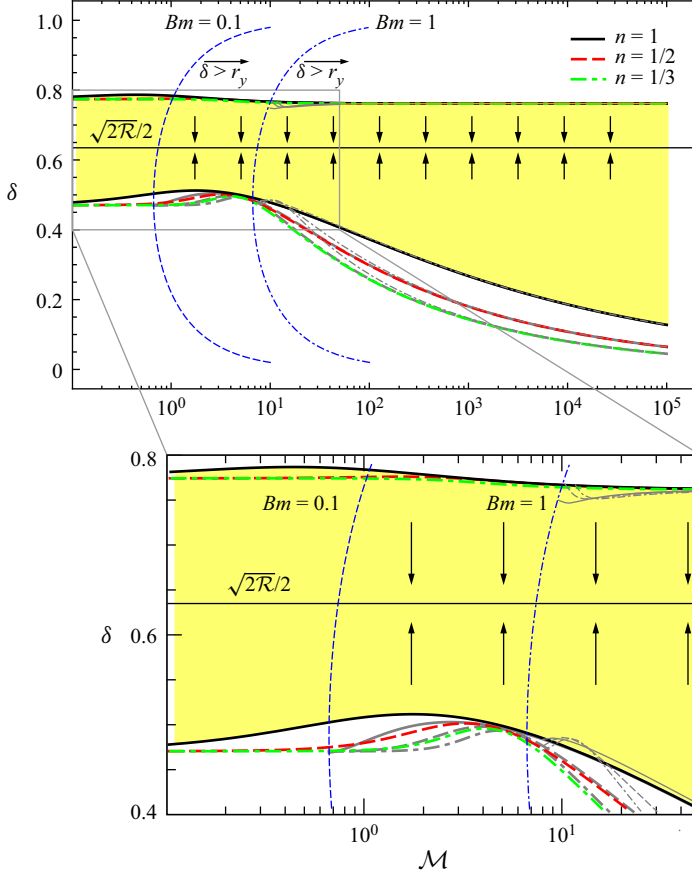
Figure 15. Domain of attraction of the stable node \delta_{3\infty} = \sqrt{2\mathcal{R}}/2 for n = 1, 1/2, 1/3 , \mathcal{R} = 0.8 , Bm = 0 (OdW fluid). The grey curves, more evident in the enlargement below, refer to a HB fluid with Bm = 0.1 (thick grey) and to Bm = 1.0 (thin grey), the blue dashed and dot-dashed curves represent the condition \delta > r_y for Bm = 0.1, 1.0 , respectively. The vertical arrows indicate the direction of evolution over time of the radius of the ascending current towards the stable node \delta_{3\infty} = \sqrt{2\mathcal{R}}/2 .
