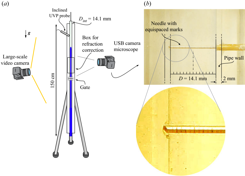
Figure 18. Experimental set-up. (a) Vertical pipe with the USB microscope camera and the video camera for large-scale image analysis; (b) a photo of the pipe, as seen from the USB camera microscope, containing glycerol and inserted in the box filled with glycerol, in order to correct the image distortion. The needle with a series of equispaced marks shows the efficiency of the distortion correction. See also the enlargement.
